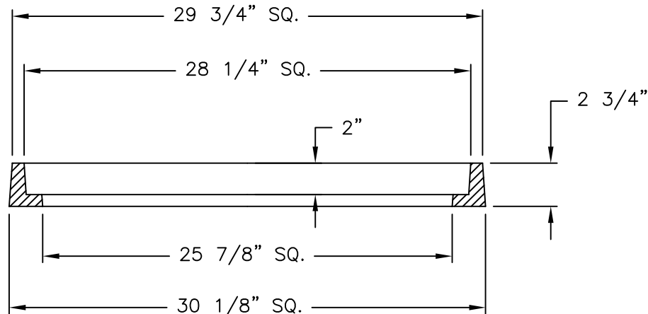
FRAME SECTION
